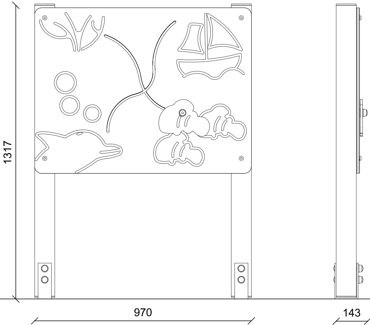
INGOMBRO MAX (OVERALL DIMENSIONS)
